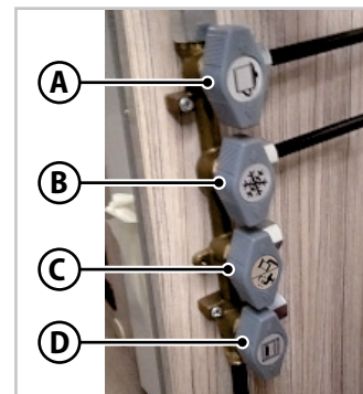
Fig.6.24 - Gasdistributionskranar
